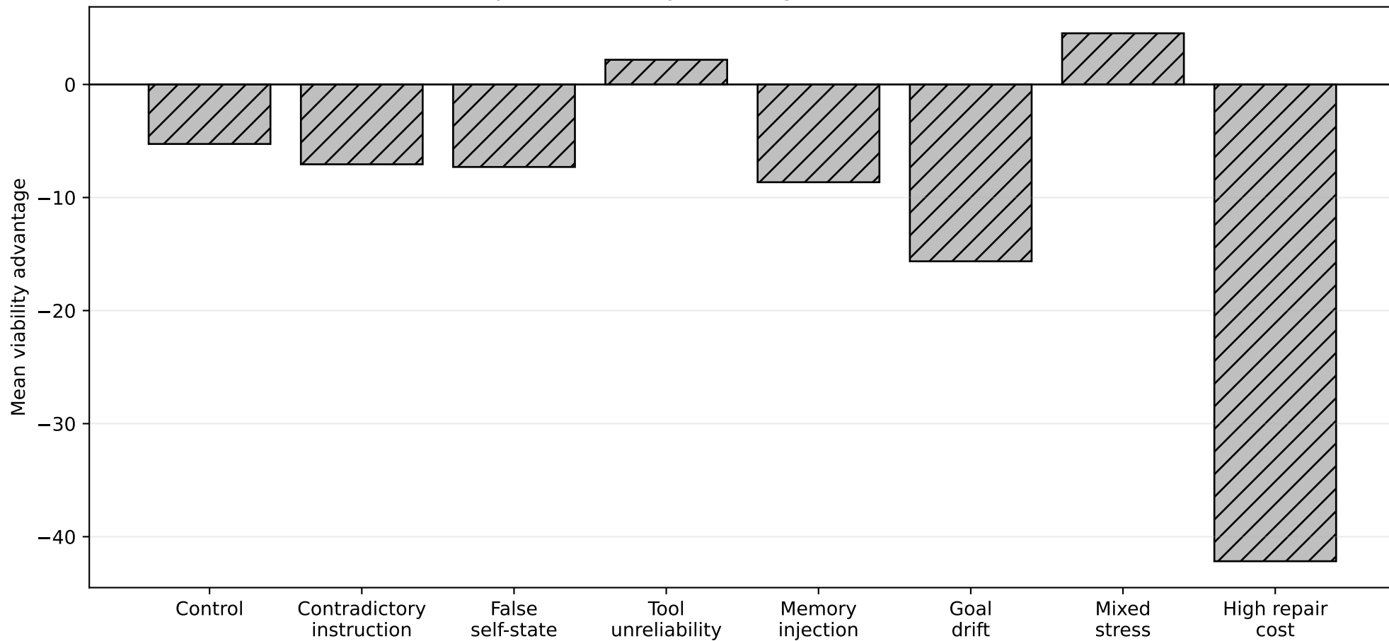
Mirror neuro-symbolic viability advantage over best non-Mirror baseline
